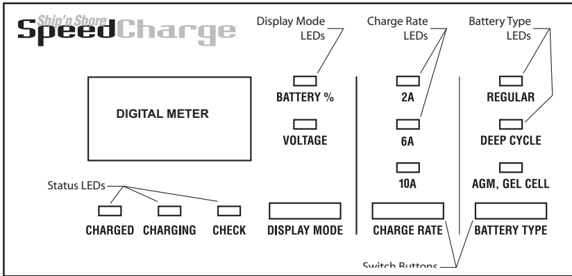
SSC-1000A CONTROL PANEL
